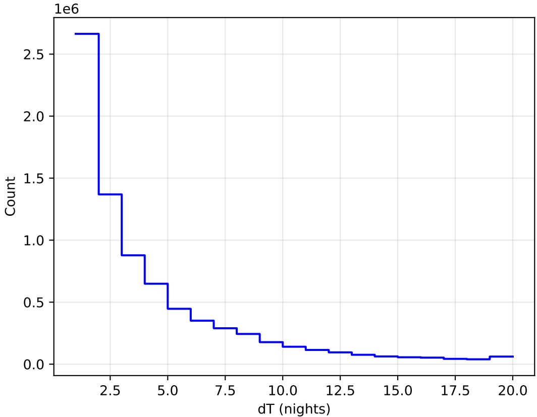
ddf_acor_sf25_lsf40_lsr20_v3.4_10yrs WFD all bands: DeltaNight Histogram
