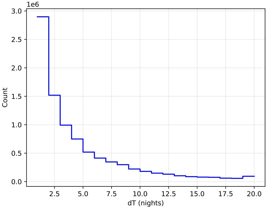
ddf_acor_sf25_lsf40_lsr20_v3.4_10yrs All sky all bands: DeltaNight Histogram
