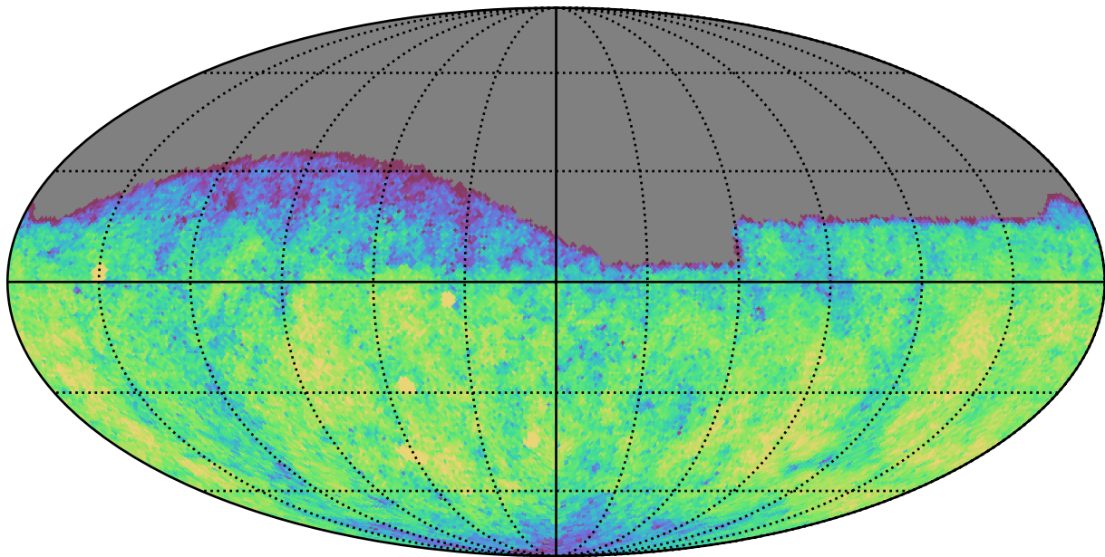
ddf_acor_sf25_lsf40_lsr20_v3.4_10yrs Yr 1 g band: CoaddM5
