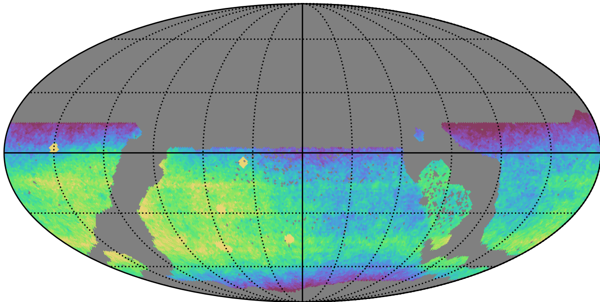
ddf_acor_sf25_lsf40_lsr20_v3.4_10yrs WFD r band: CoaddM5
