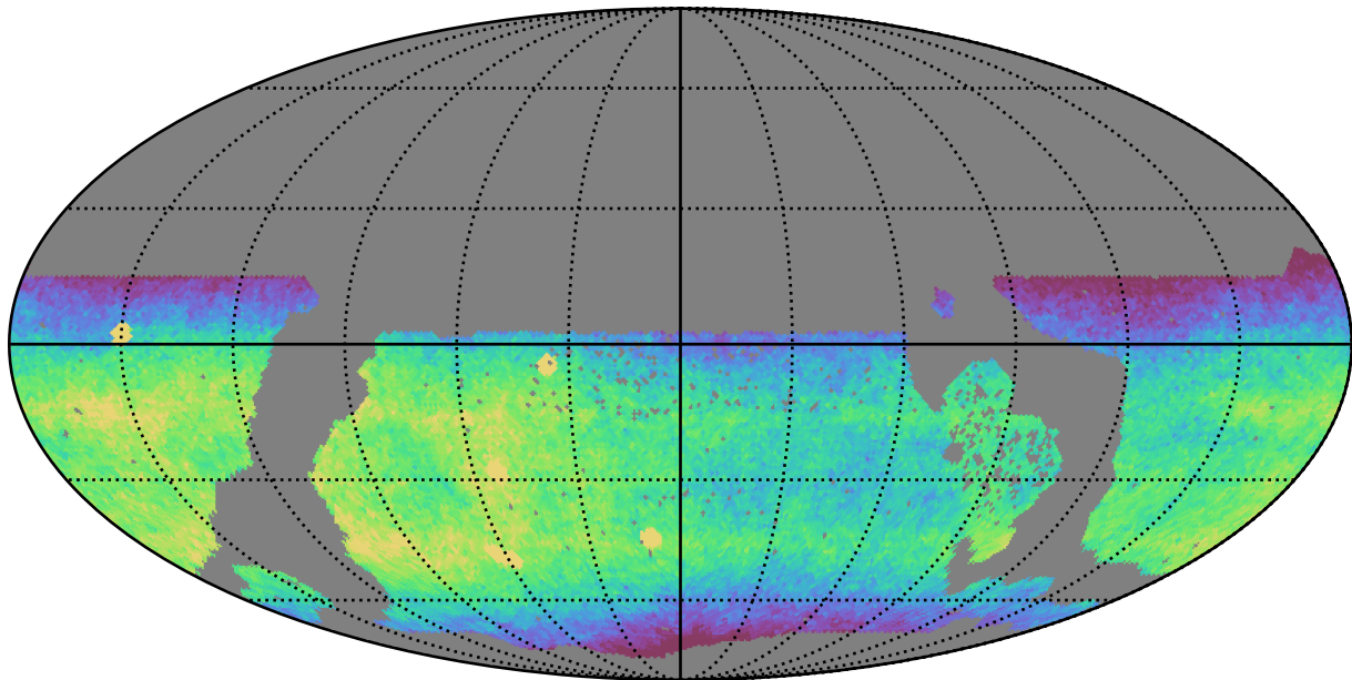
ddf_acor_sf25_lsf40_lsr20_v3.4_10yrs WFD i band: CoaddM5
