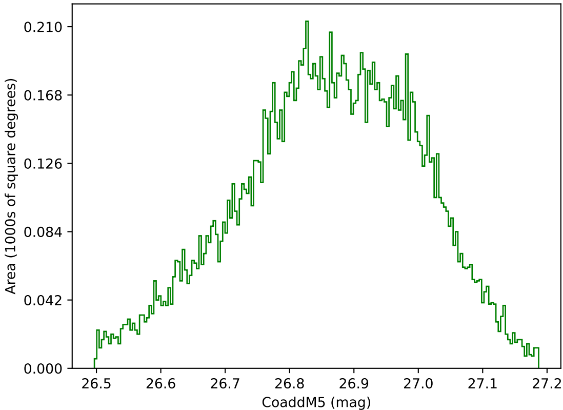
ddf_acor_sf25_lsf40_lsr20_v3.4_10yrs WFD g band: CoaddM5
