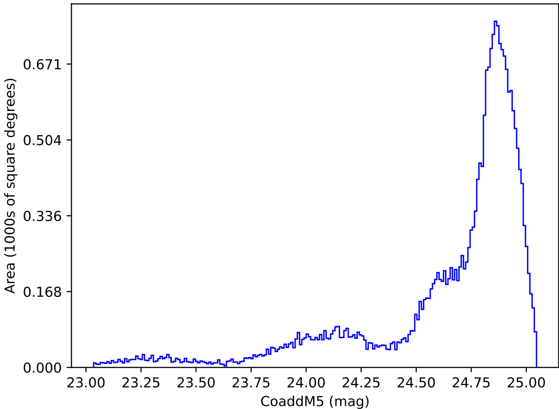
ddf_acor_sf25_lsf40_lsr20_v3.4_10yrs All sky y band: CoaddM5
