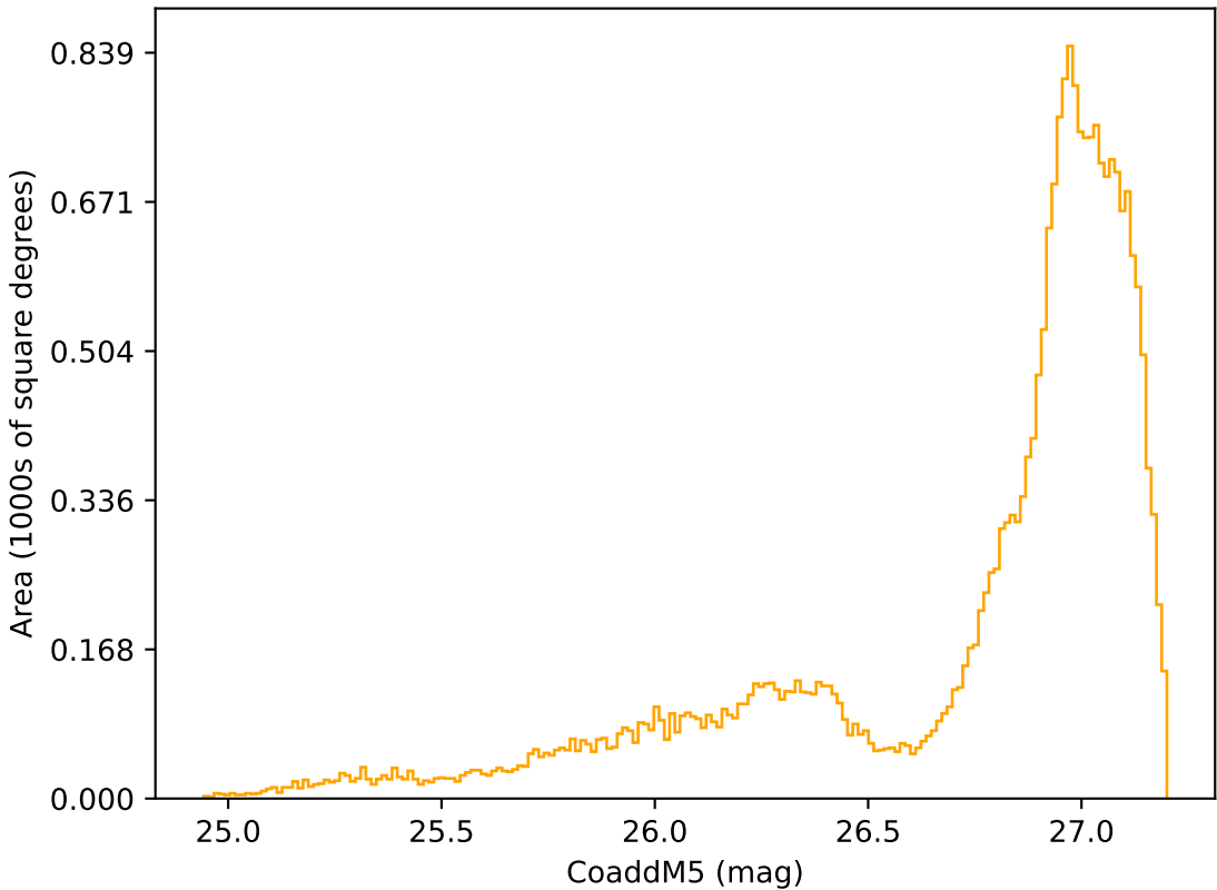
ddf_acor_sf25_lsf40_lsr20_v3.4_10yrs All sky r band: CoaddM5
