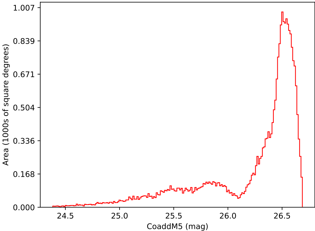
ddf_acor_sf25_lsf40_lsr20_v3.4_10yrs All sky i band: CoaddM5
