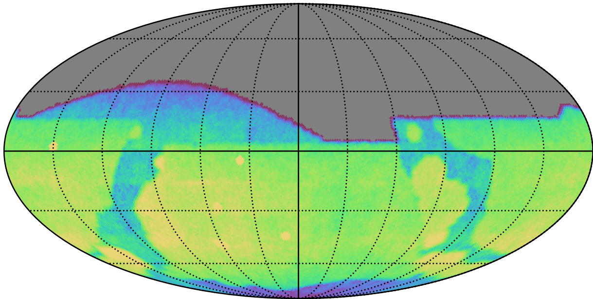
ddf_acor_sf25_lsf40_lsr20_v3.4_10yrs All sky g band: CoaddM5
