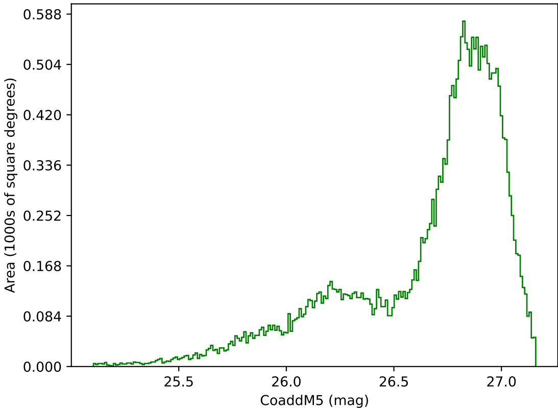
ddf_acor_sf25_lsf40_lsr20_v3.4_10yrs All sky g band: CoaddM5
