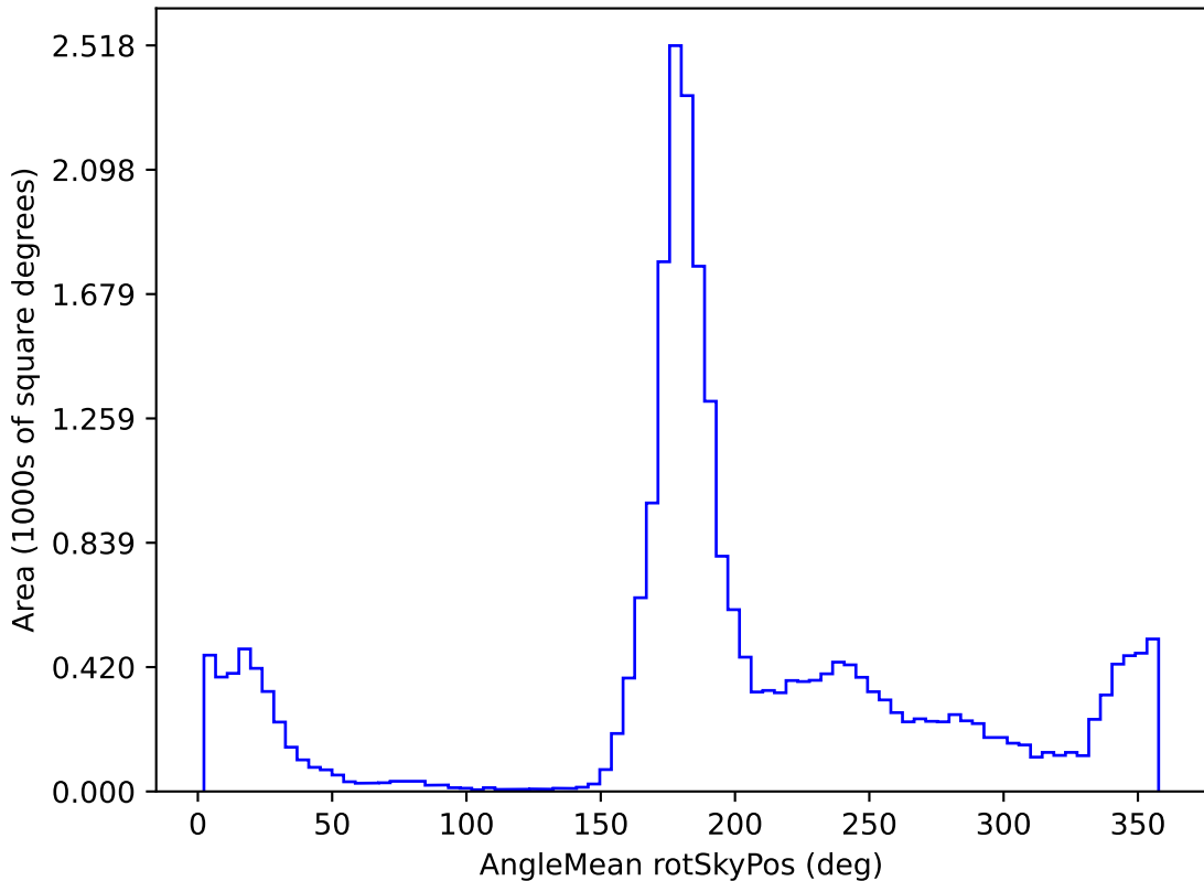
ddf_acor_sf25_lsf40_lsr20_v3.4_10yrs All sky r band: AngleMean rotSkyPos
