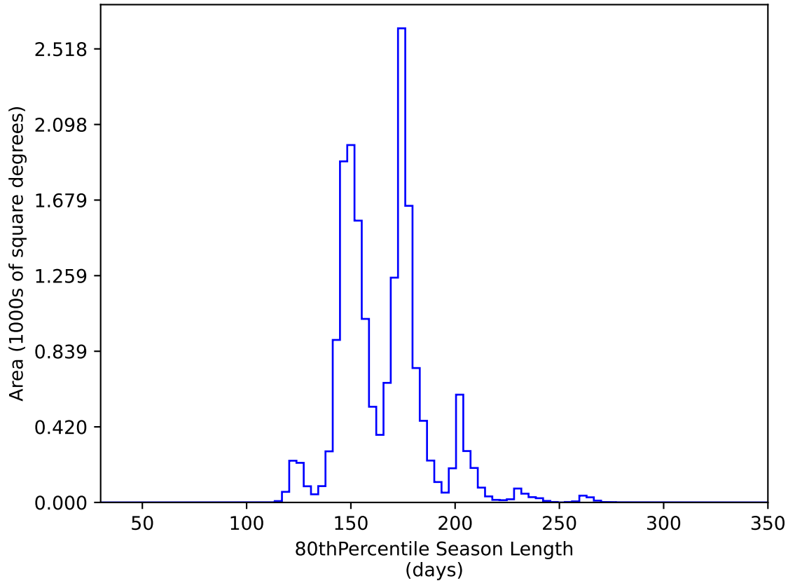
ddf_acor_sf25_lsf40_lsr20_v3.4_10yrs WFD y band: 80thPercentile Season Length
