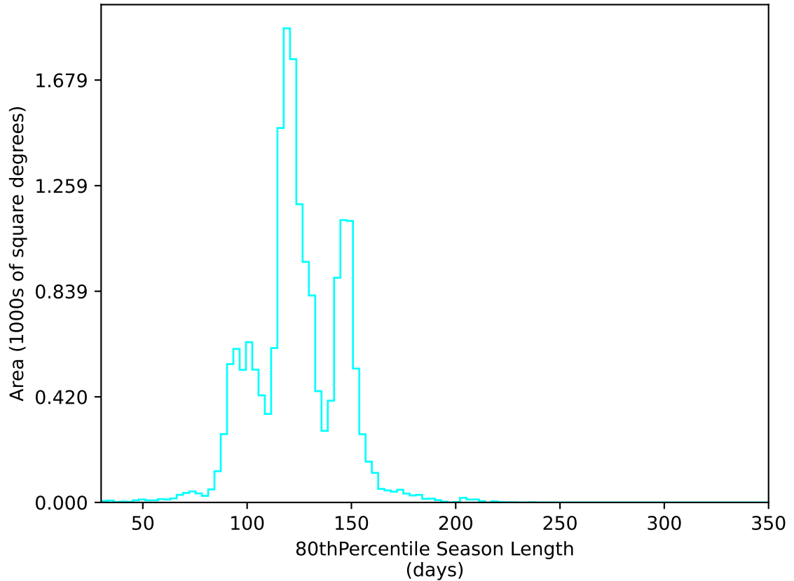
ddf_acor_sf25_lsf40_lsr20_v3.4_10yrs WFD u band: 80thPercentile Season Length
