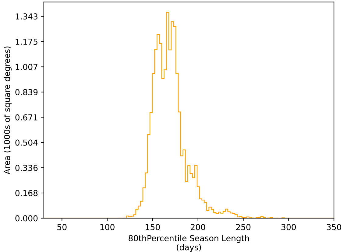
ddf_acor_sf25_lsf40_lsr20_v3.4_10yrs WFD r band: 80thPercentile Season Length
