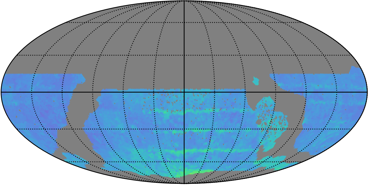
ddf_acor_sf25_lsf40_lsr20_v3.4_10yrs WFD i band: 80thPercentile Season Length
