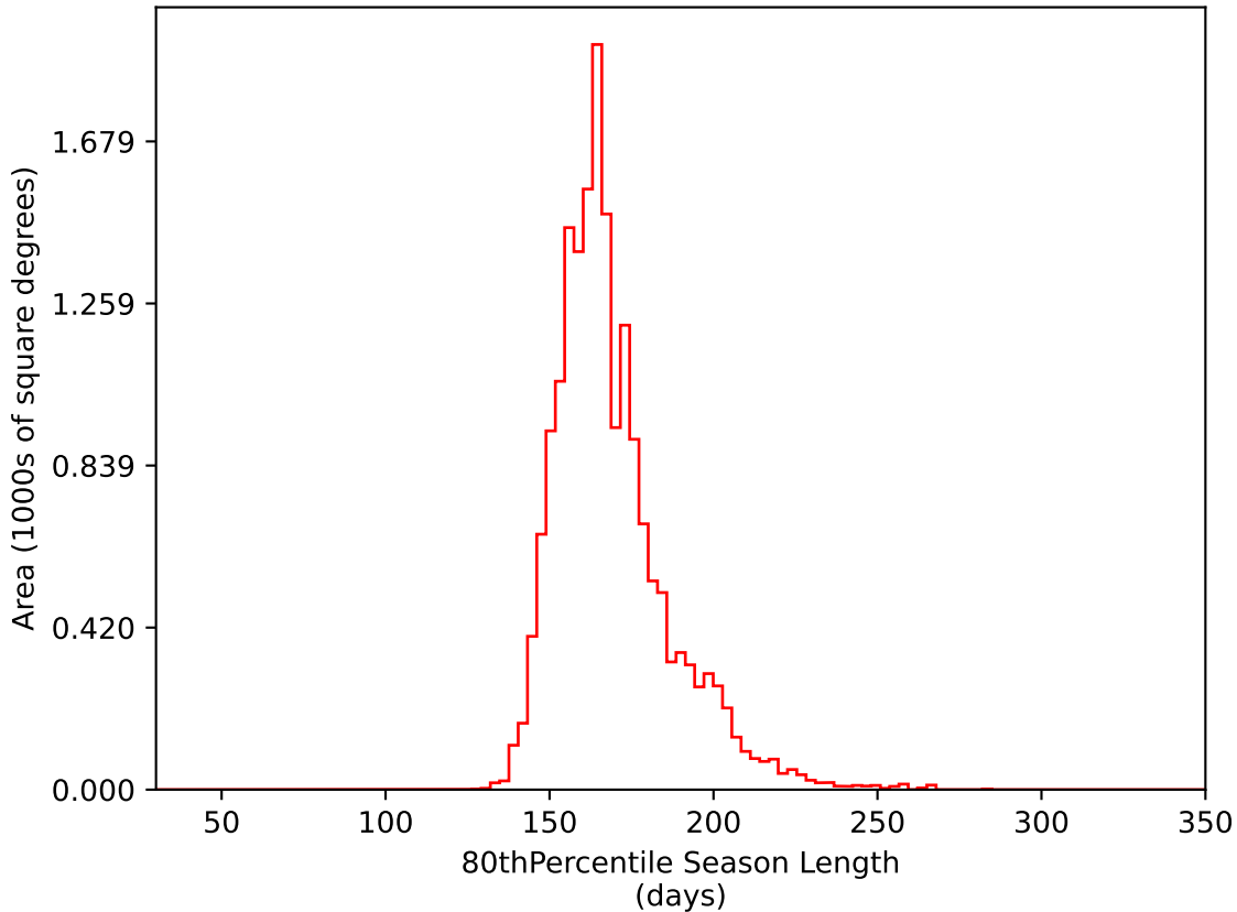
ddf_acor_sf25_lsf40_lsr20_v3.4_10yrs WFD i band: 80thPercentile Season Length
