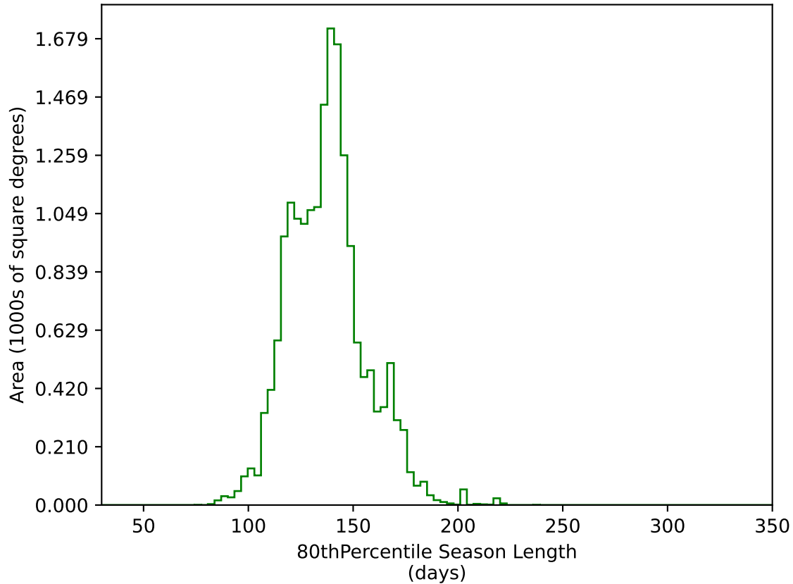
ddf_acor_sf25_lsf40_lsr20_v3.4_10yrs WFD g band: 80thPercentile Season Length
