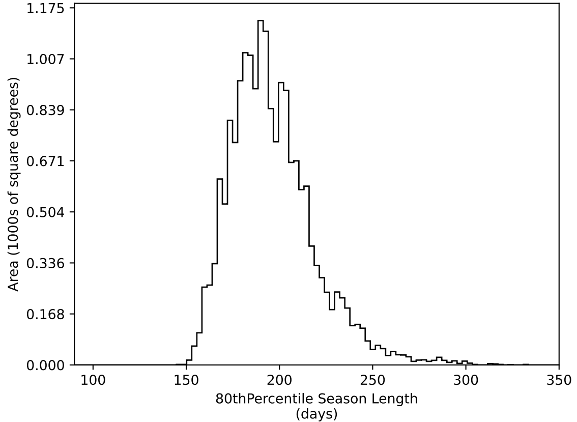
ddf_acor_sf25_lsf40_lsr20_v3.4_10yrs WFD all bands: 80thPercentile Season Length
