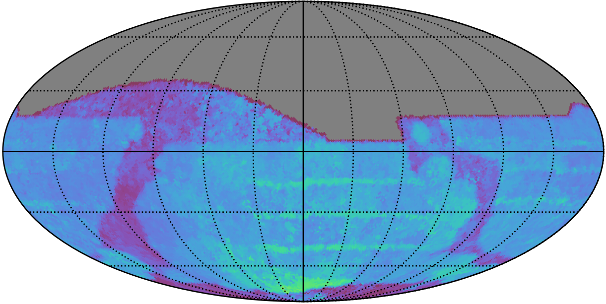
ddf_acor_sf25_lsf40_lsr20_v3.4_10yrs All sky z band: 80thPercentile Season Length
