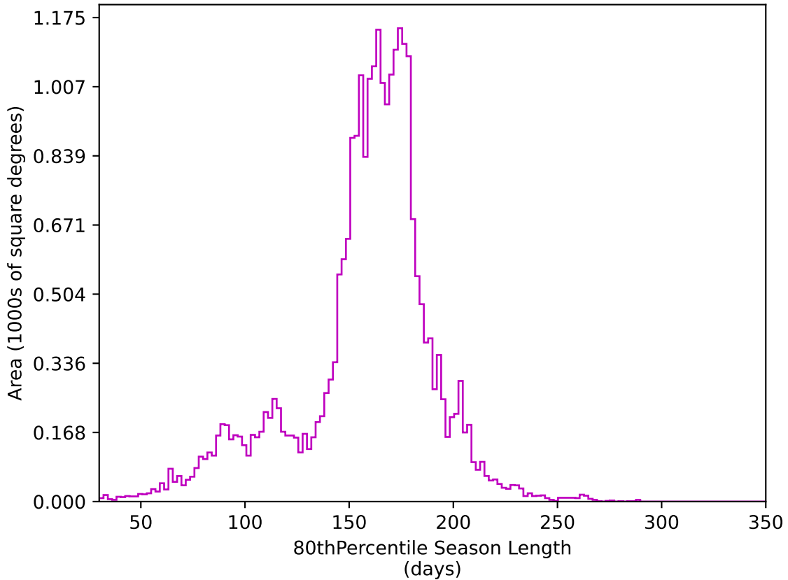
ddf_acor_sf25_lsf40_lsr20_v3.4_10yrs All sky z band: 80thPercentile Season Length
