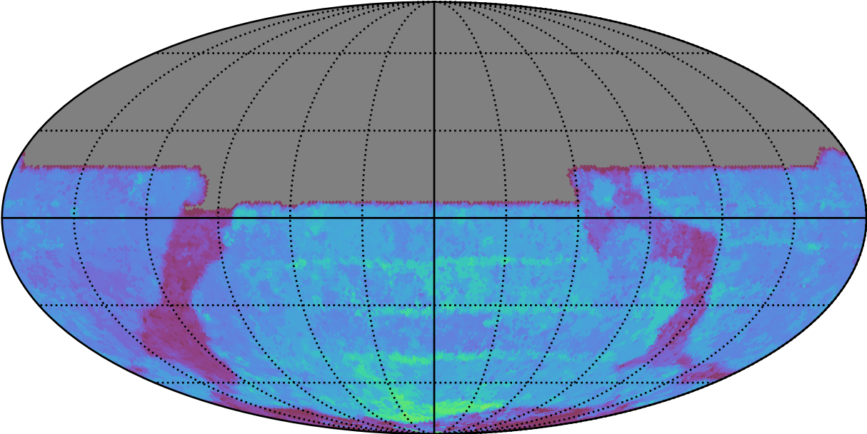
ddf_acor_sf25_lsf40_lsr20_v3.4_10yrs All sky y band: 80thPercentile Season Length
