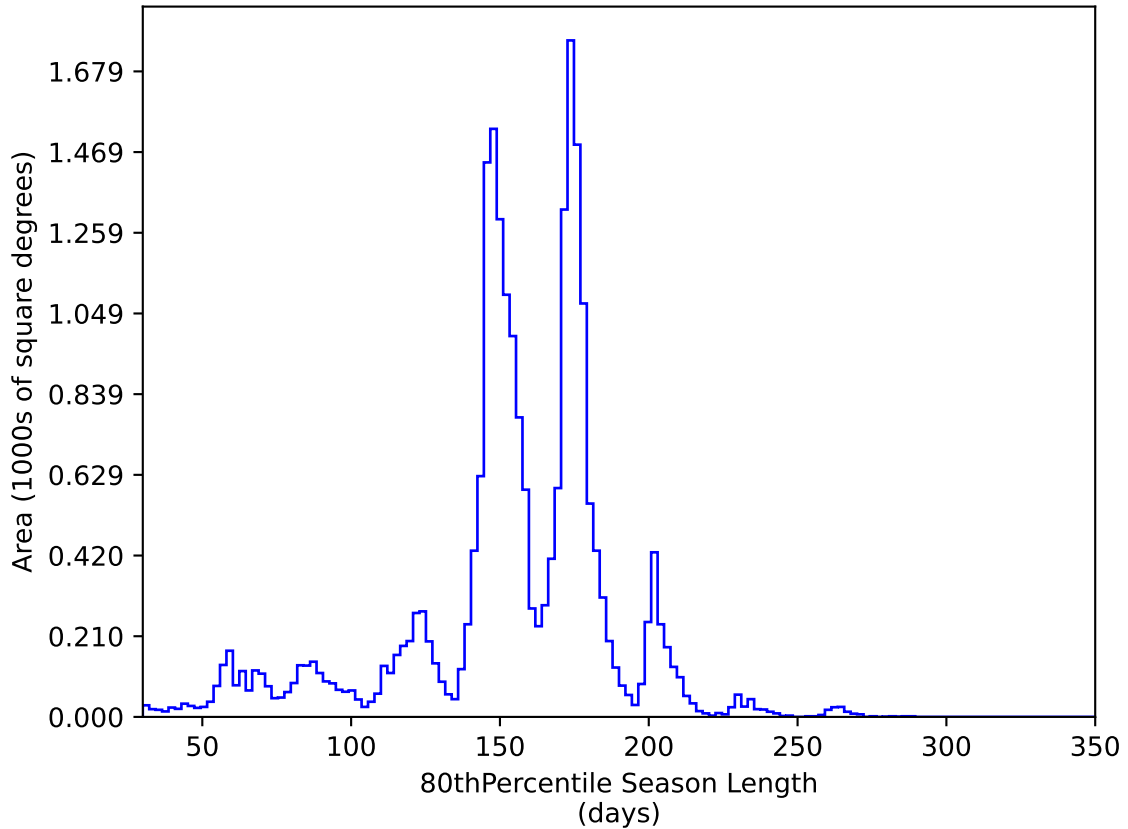
ddf_acor_sf25_lsf40_lsr20_v3.4_10yrs All sky y band: 80thPercentile Season Length
