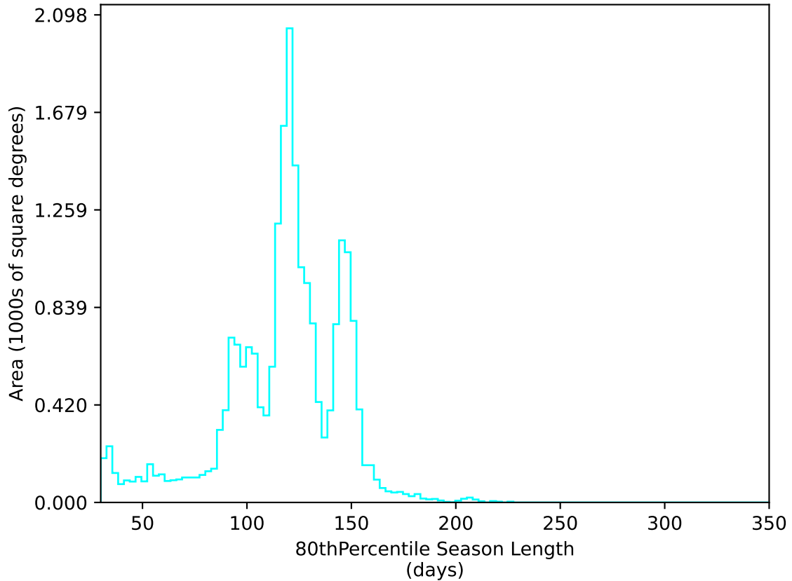
ddf_acor_sf25_lsf40_lsr20_v3.4_10yrs All sky u band: 80thPercentile Season Length
