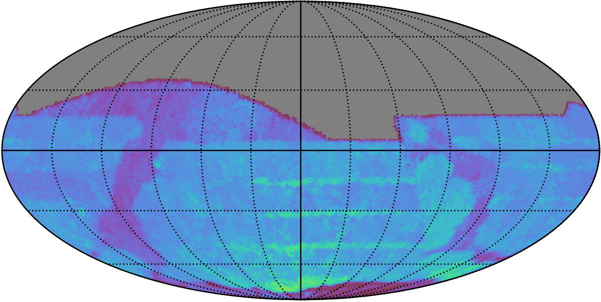
ddf_acor_sf25_lsf40_lsr20_v3.4_10yrs All sky r band: 80thPercentile Season Length
