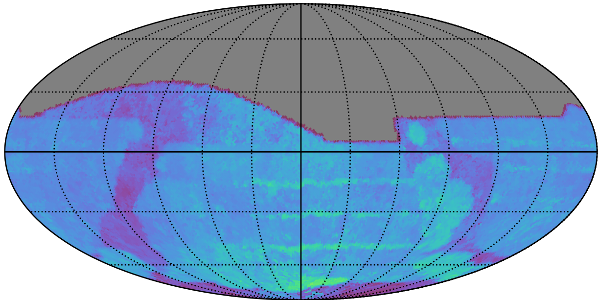
ddf_acor_sf25_lsf40_lsr20_v3.4_10yrs All sky i band: 80thPercentile Season Length
