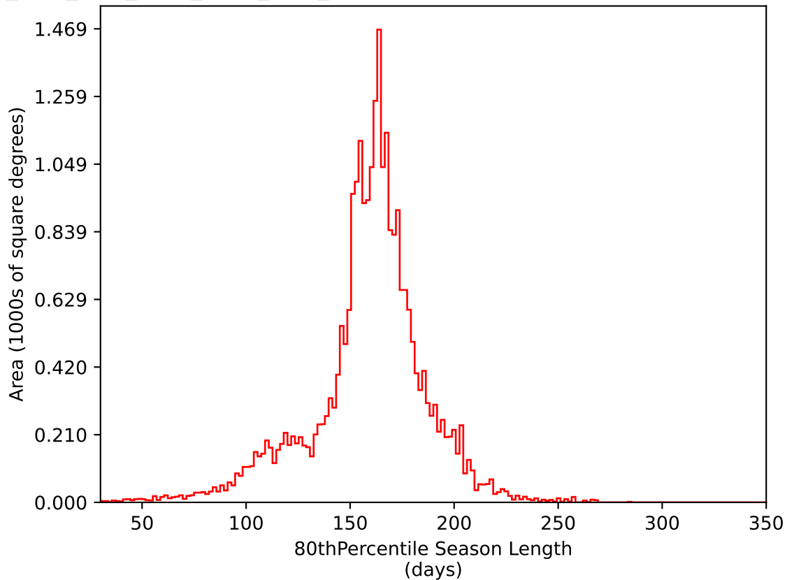
ddf_acor_sf25_lsf40_lsr20_v3.4_10yrs All sky i band: 80thPercentile Season Length
