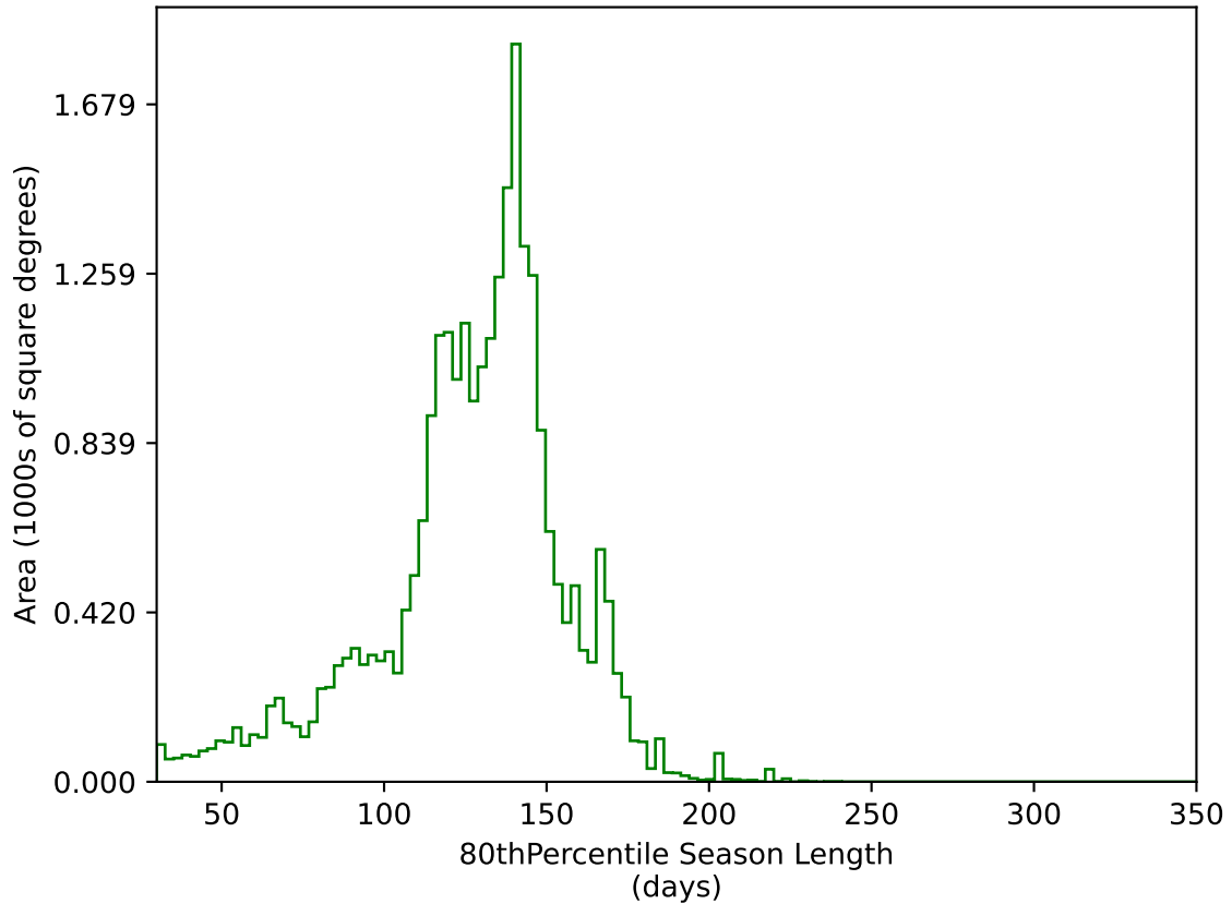
ddf_acor_sf25_lsf40_lsr20_v3.4_10yrs All sky g band: 80thPercentile Season Length
