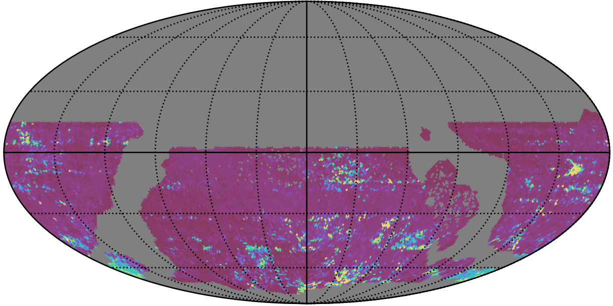
ddf_acor_sf25_lsf40_lsr20_v3.4_10yrs WFD z band: 75th Percentile Intranight Timespan
