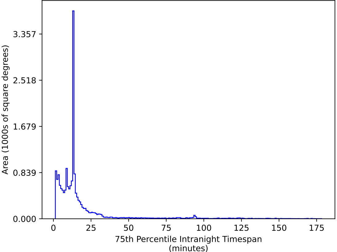
ddf_acor_sf25_lsf40_lsr20_v3.4_10yrs WFD z band: 75th Percentile Intranight Timespan
