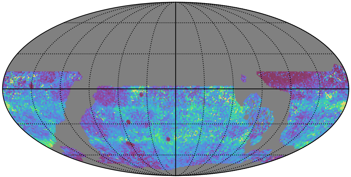
ddf_acor_sf25_lsf40_lsr20_v3.4_10yrs WFD y band: 75th Percentile Intranight Timespan
