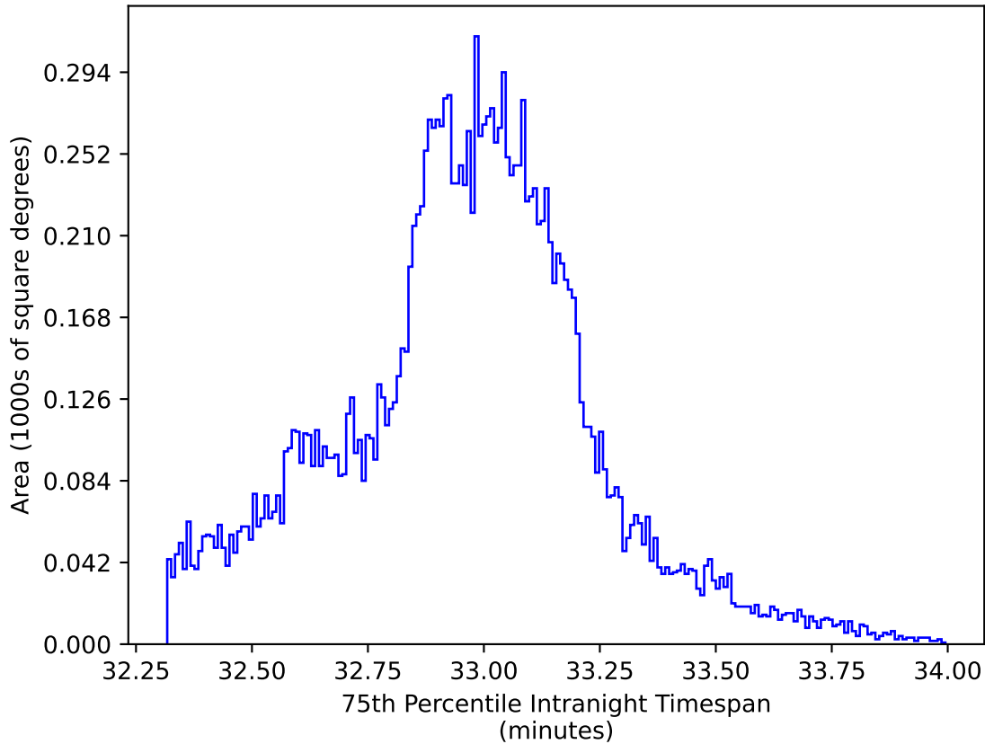
ddf_acor_sf25_lsf40_lsr20_v3.4_10yrs WFD y band: 75th Percentile Intranight Timespan
