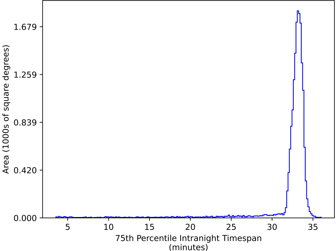
ddf_acor_sf25_lsf40_lsr20_v3.4_10yrs WFD ug bands: 75th Percentile Intranight Timespan
