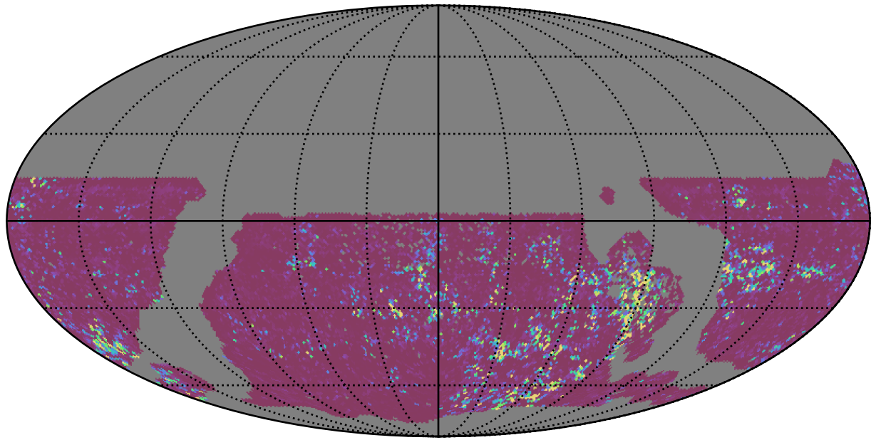
ddf_acor_sf25_lsf40_lsr20_v3.4_10yrs WFD u band: 75th Percentile Intranight Timespan
