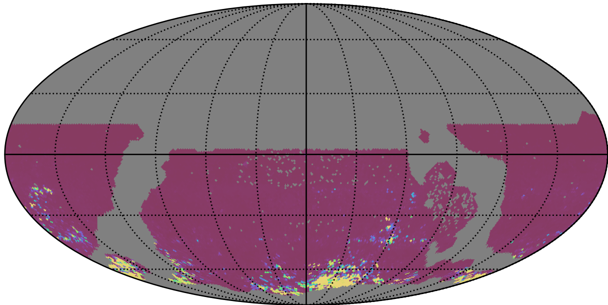
ddf_acor_sf25_lsf40_lsr20_v3.4_10yrs WFD ri bands: 75th Percentile Intranight Timespan
