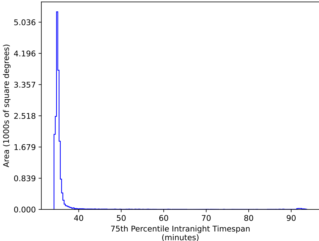
ddf_acor_sf25_lsf40_lsr20_v3.4_10yrs WFD ri bands: 75th Percentile Intranight Timespan
