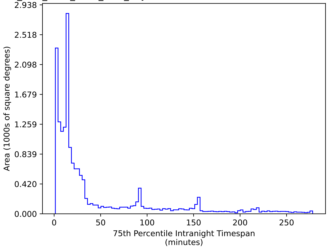
ddf_acor_sf25_lsf40_lsr20_v3.4_10yrs WFD r band: 75th Percentile Intranight Timespan
