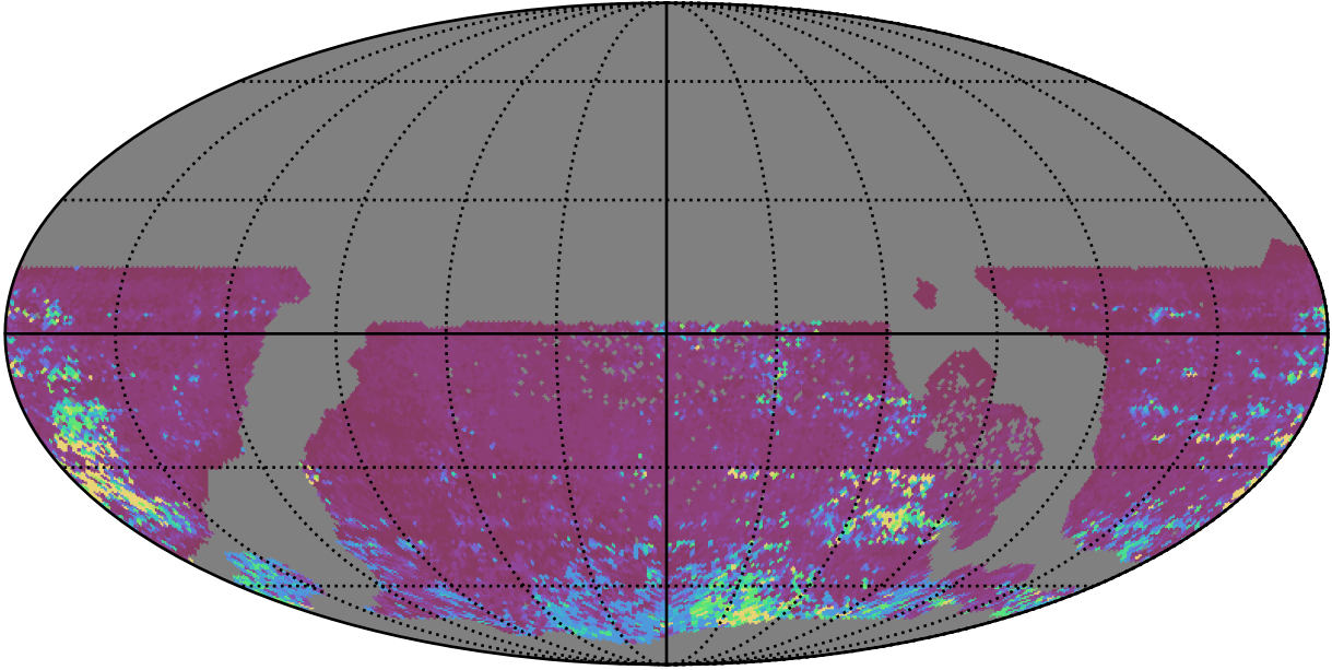
ddf_acor_sf25_lsf40_lsr20_v3.4_10yrs WFD i band: 75th Percentile Intranight Timespan
