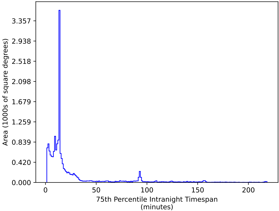
ddf_acor_sf25_lsf40_lsr20_v3.4_10yrs WFD i band: 75th Percentile Intranight Timespan
