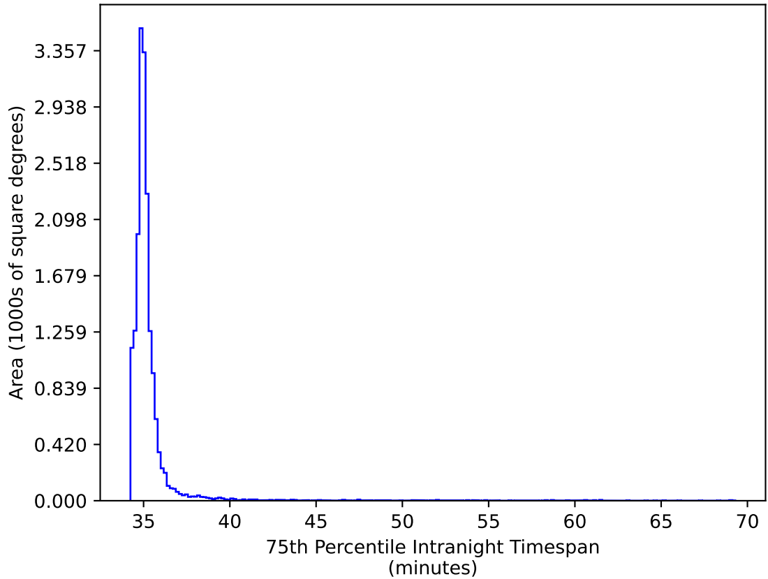
ddf_acor_sf25_lsf40_lsr20_v3.4_10yrs WFD gr bands: 75th Percentile Intranight Timespan
