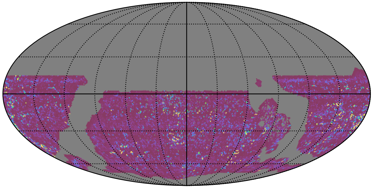
ddf_acor_sf25_lsf40_lsr20_v3.4_10yrs WFD g band: 75th Percentile Intranight Timespan
