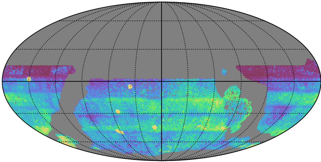
ddf_acor_sf25_lsf40_lsr20_v3.4_10yrs WFD all bands: 75th Percentile Intranight Timespan
