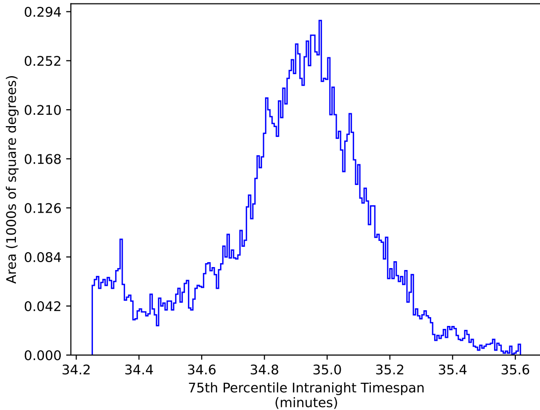
ddf_acor_sf25_Isf40_Isr20_v3.4_10yrs WFD all bands: 75th Percentile Intranight Timespan
