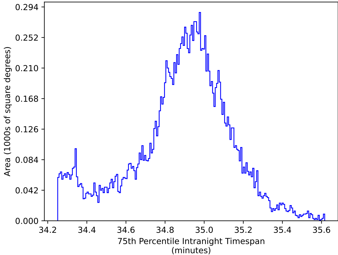
ddf_acor_sf25_lsf40_lsr20_v3.4_10yrs WFD: 75th Percentile Intranight Timespan
