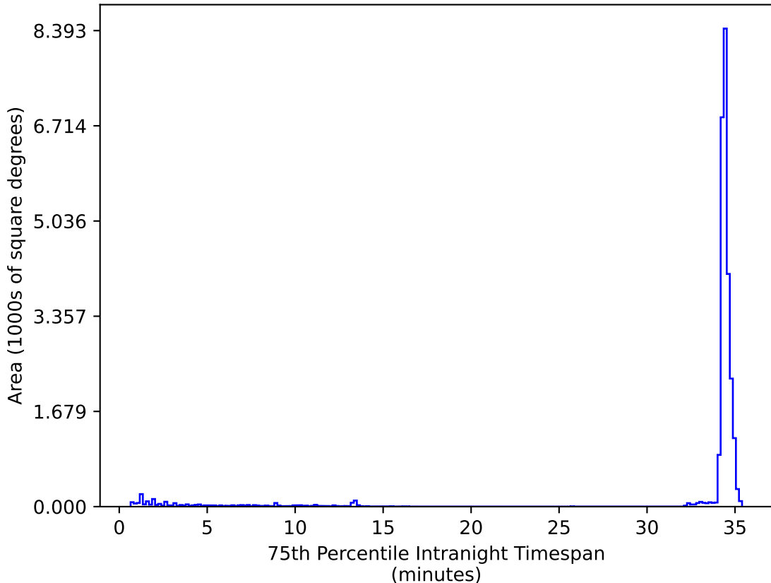
ddf_acor_sf25_lsf40_lsr20_v3.4_10yrs All sky zy bands: 75th Percentile Intranight Timespan
