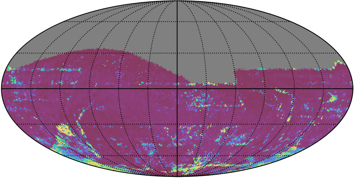
ddf_acor_sf25_lsf40_lsr20_v3.4_10yrs All sky z band: 75th Percentile Intranight Timespan
