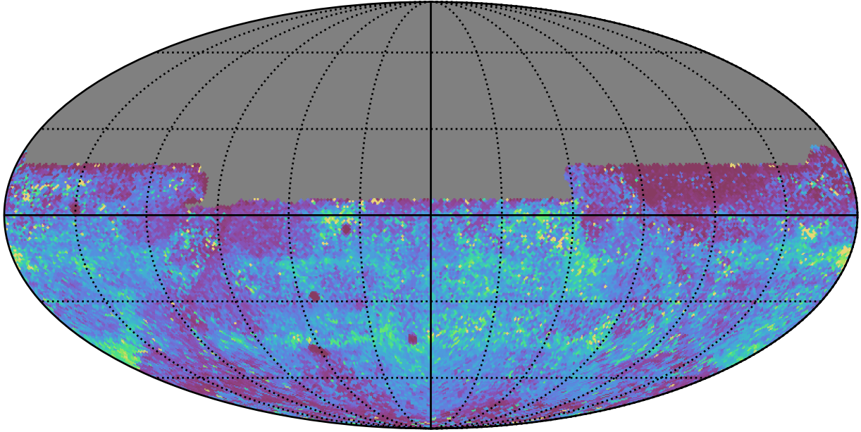
ddf_acor_sf25_lsf40_lsr20_v3.4_10yrs All sky y band: 75th Percentile Intranight Timespan
