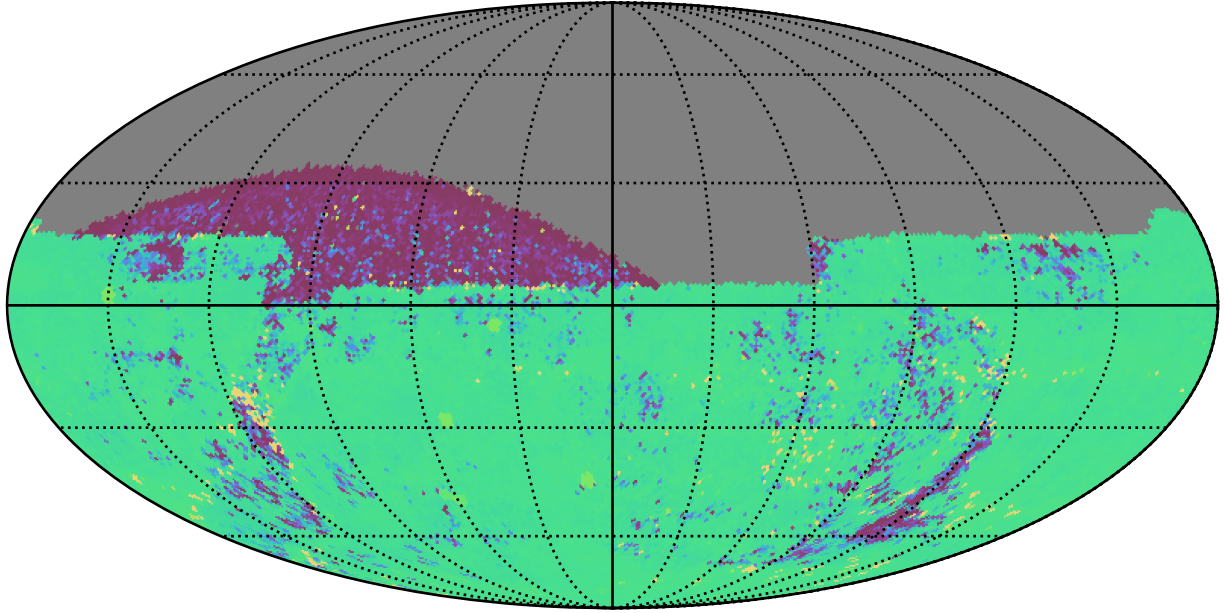
ddf_acor_sf25_lsf40_lsr20_v3.4_10yrs All sky ug bands: 75th Percentile Intranight Timespan
