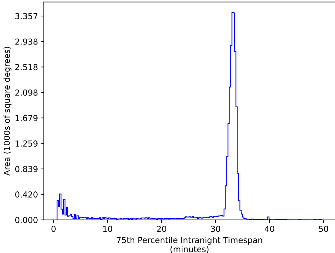
ddf_acor_sf25_lsf40_lsr20_v3.4_10yrs All sky ug bands: 75th Percentile Intranight Timespan
