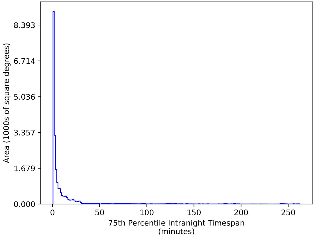
ddf_acor_sf25_lsf40_lsr20_v3.4_10yrs All sky u band: 75th Percentile Intranight Timespan
